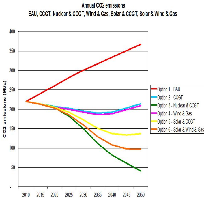
Figure 7: CO 2 emissions per year for the six options
